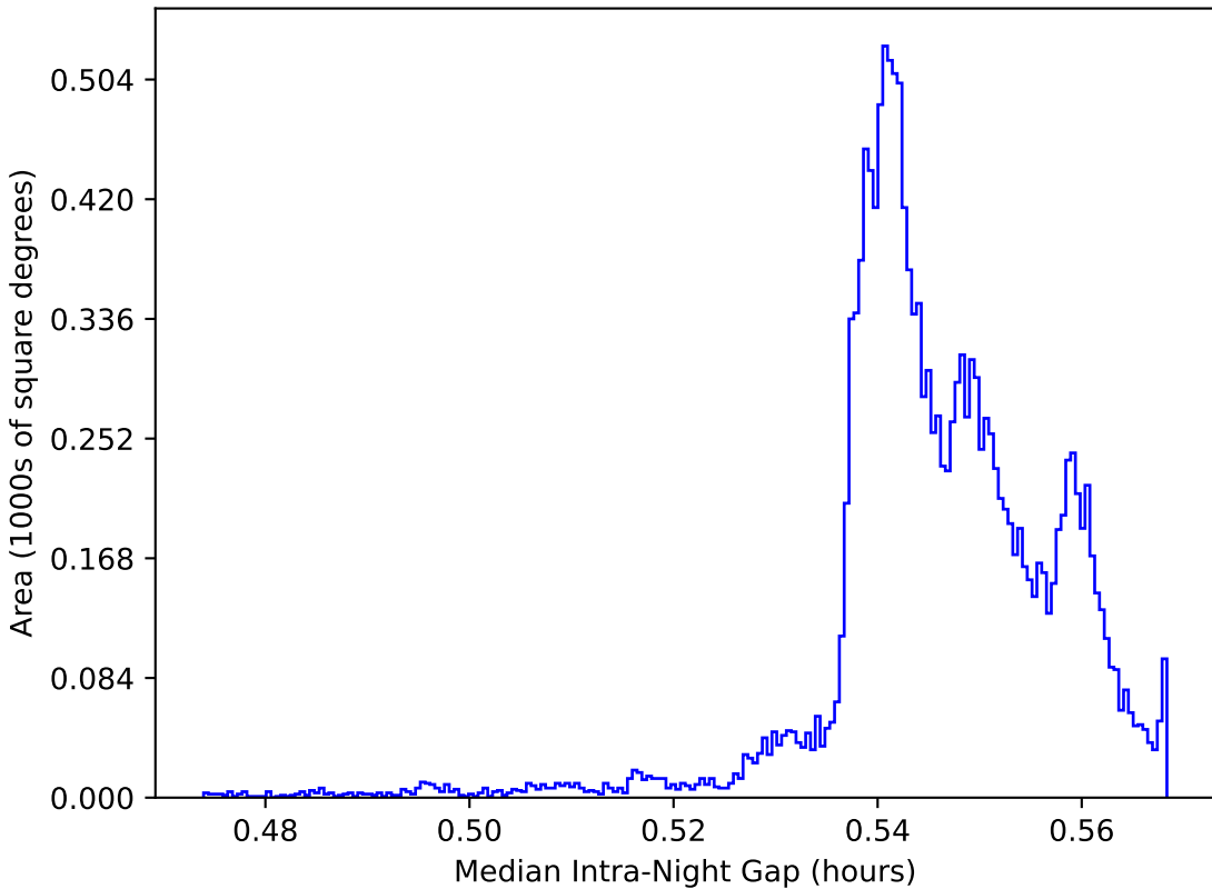
extra_ss_neo2_v3.4_10yrs WFD: Median Intra-Night Gap
