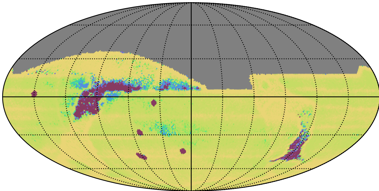
extra_ss_neo2_v3.4_10yrs All sky: Median Intra-Night Gap
