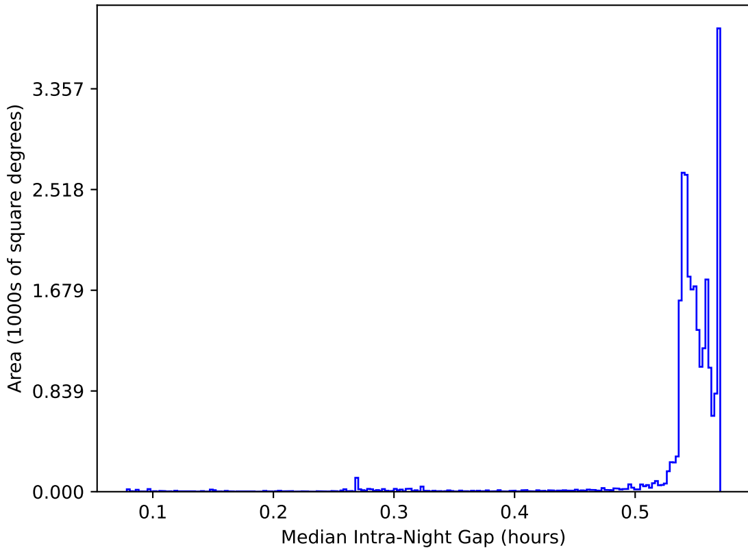
extra_ss_neo2_v3.4_10yrs All sky: Median Intra-Night Gap
