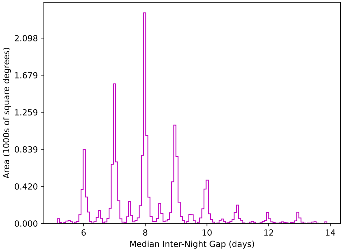
extra_ss_neo2_v3.4_10yrs WFD z band: Median Inter-Night Gap
