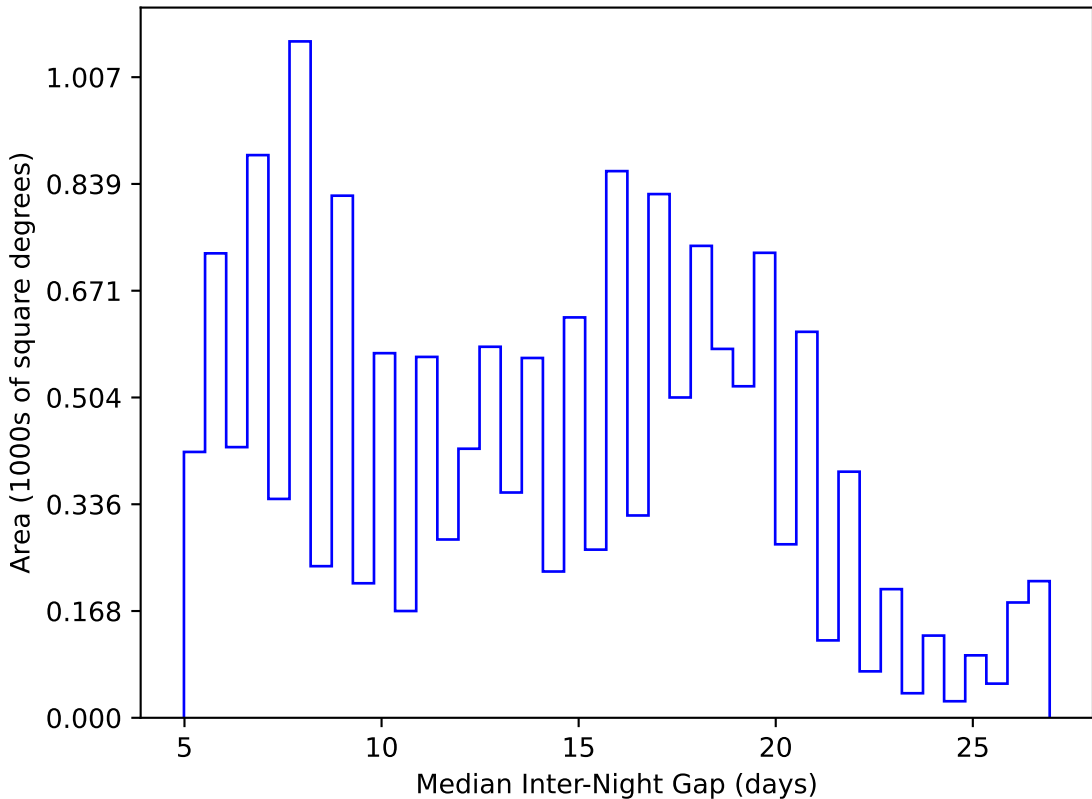
extra_ss_neo2_v3.4_10yrs WFD y band: Median Inter-Night Gap
