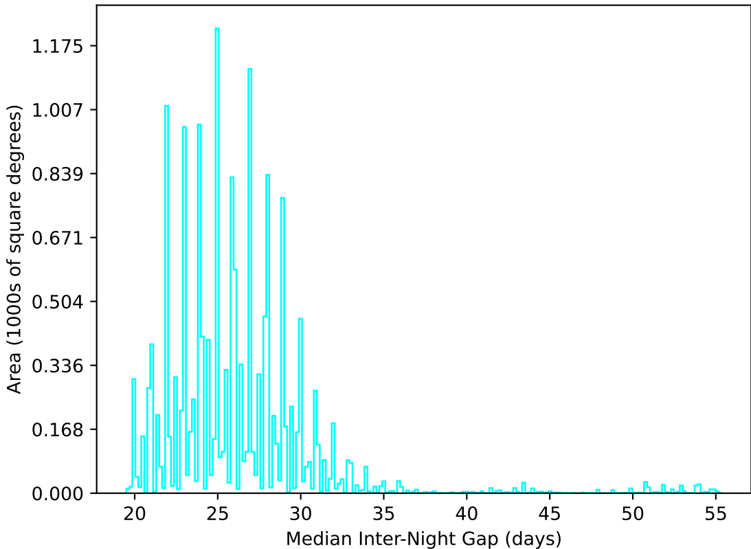
extra_ss_neo2_v3.4_10yrs WFD u band: Median Inter-Night Gap
