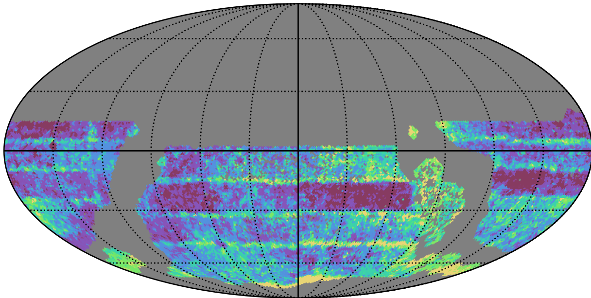
extra_ss_neo2_v3.4_10yrs WFD r band: Median Inter-Night Gap
