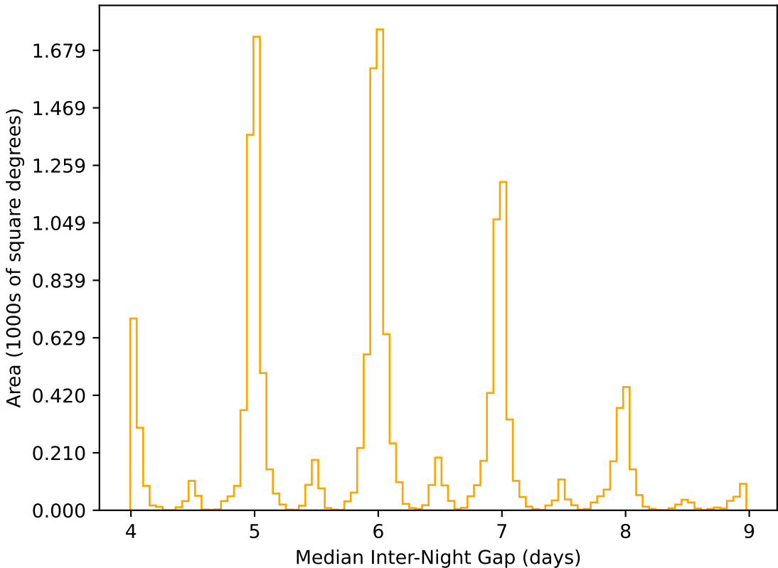
extra_ss_neo2_v3.4_10yrs WFD r band: Median Inter-Night Gap
