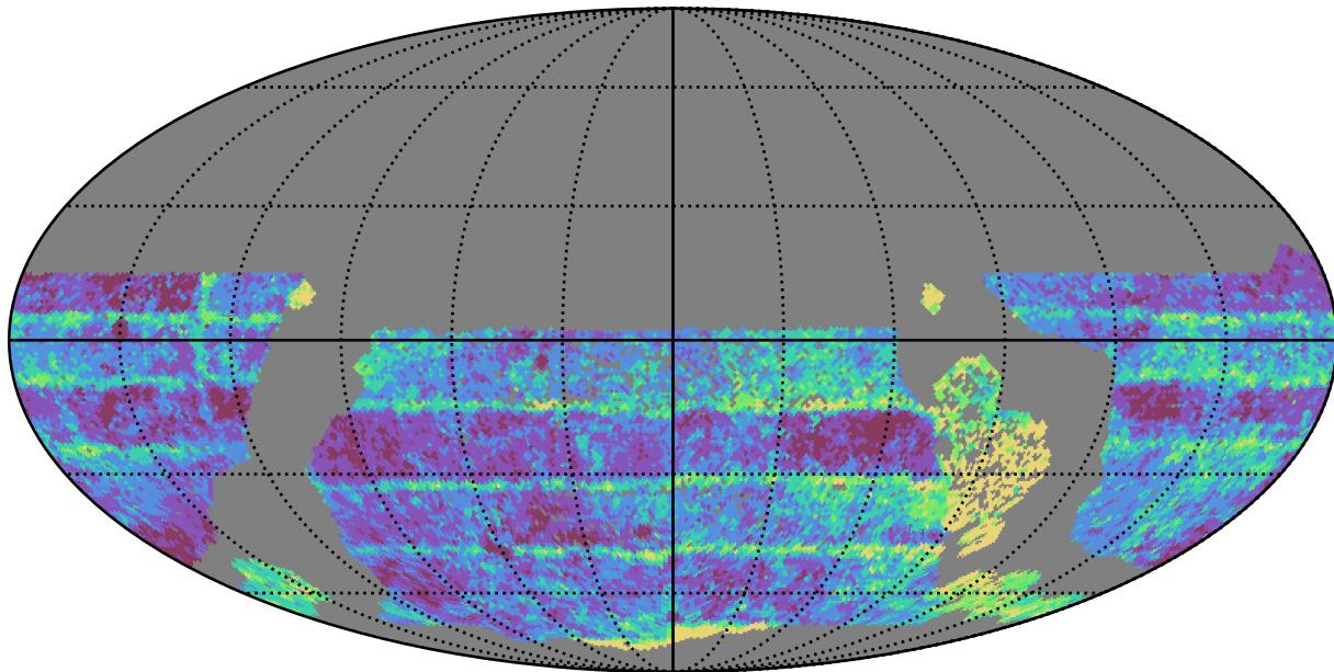
extra_ss_neo2_v3.4_10yrs WFD i band: Median Inter-Night Gap
