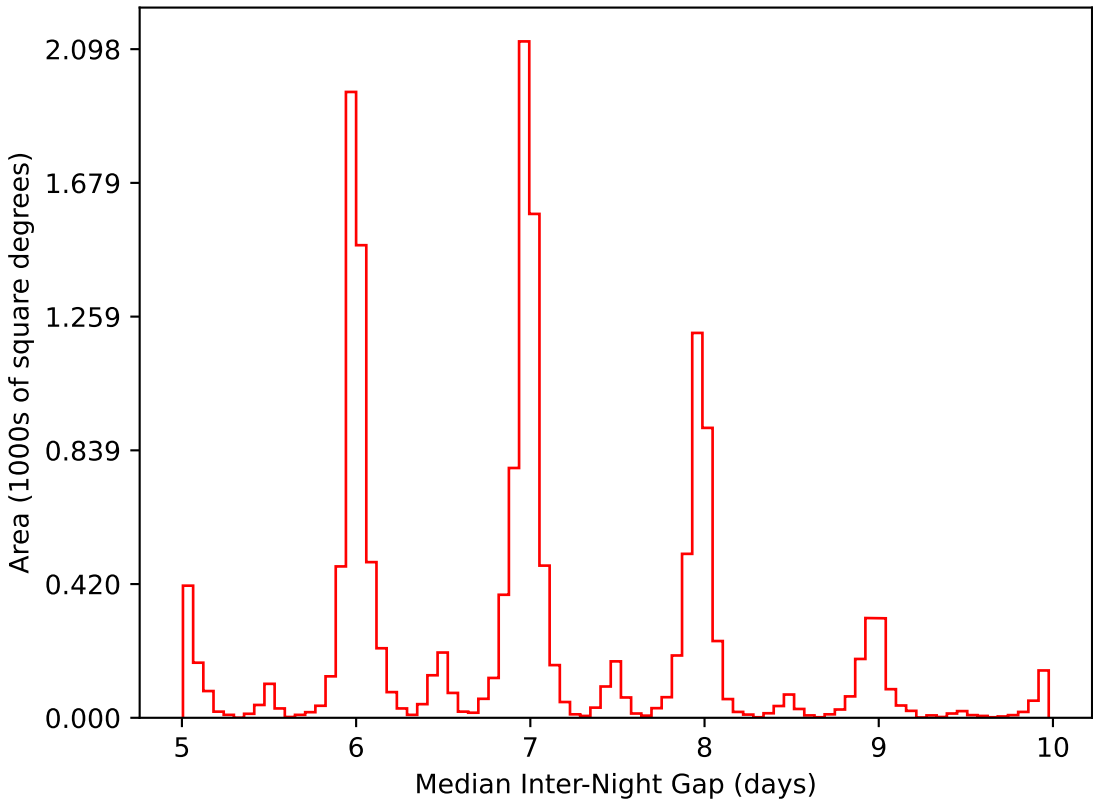
extra_ss_neo2_v3.4_10yrs WFD i band: Median Inter-Night Gap
