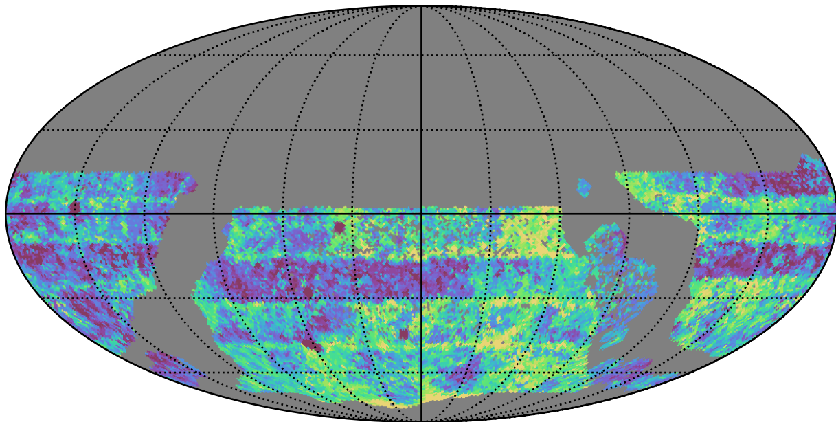
extra_ss_neo2_v3.4_10yrs WFD g band: Median Inter-Night Gap
