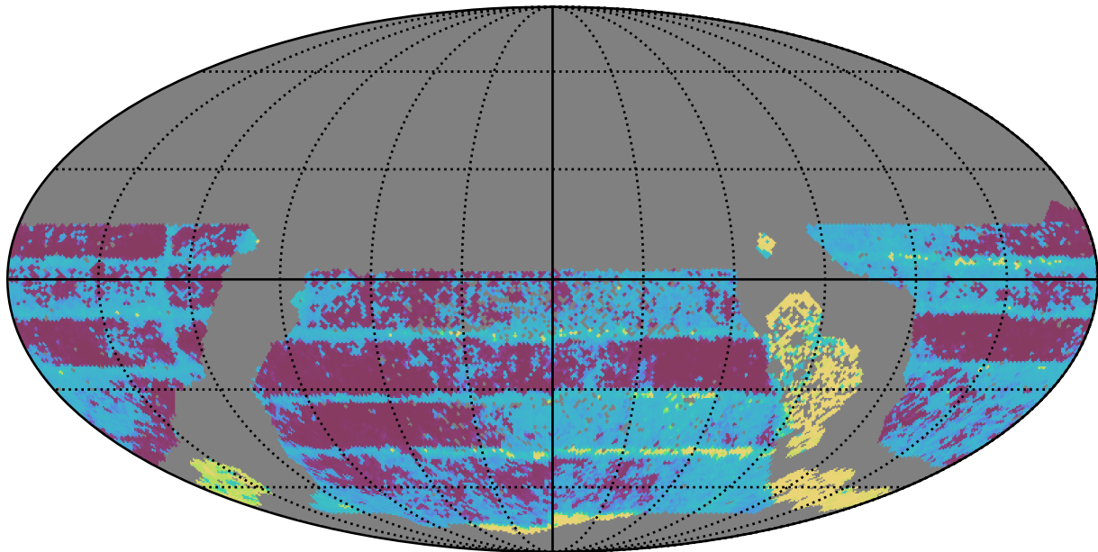
extra_ss_neo2_v3.4_10yrs WFD all bands: Median Inter-Night Gap
