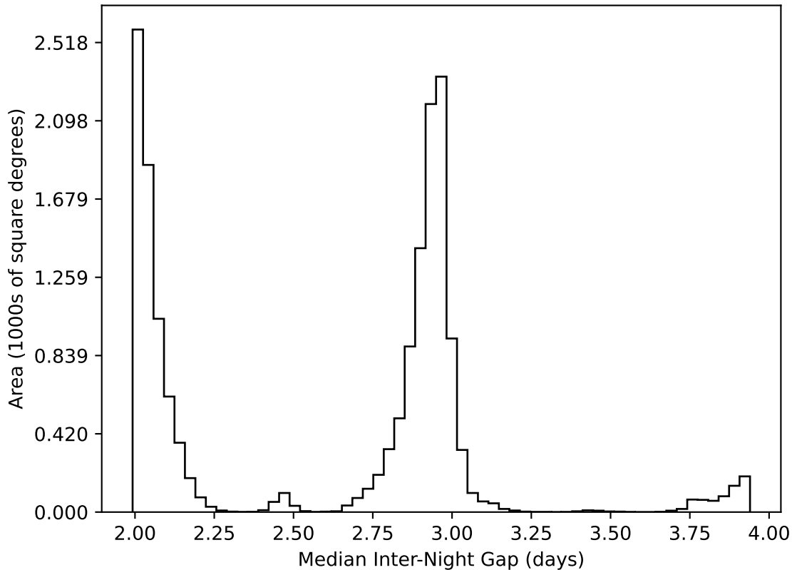
extra_ss_neo2_v3.4_10yrs WFD all bands: Median Inter-Night Gap
