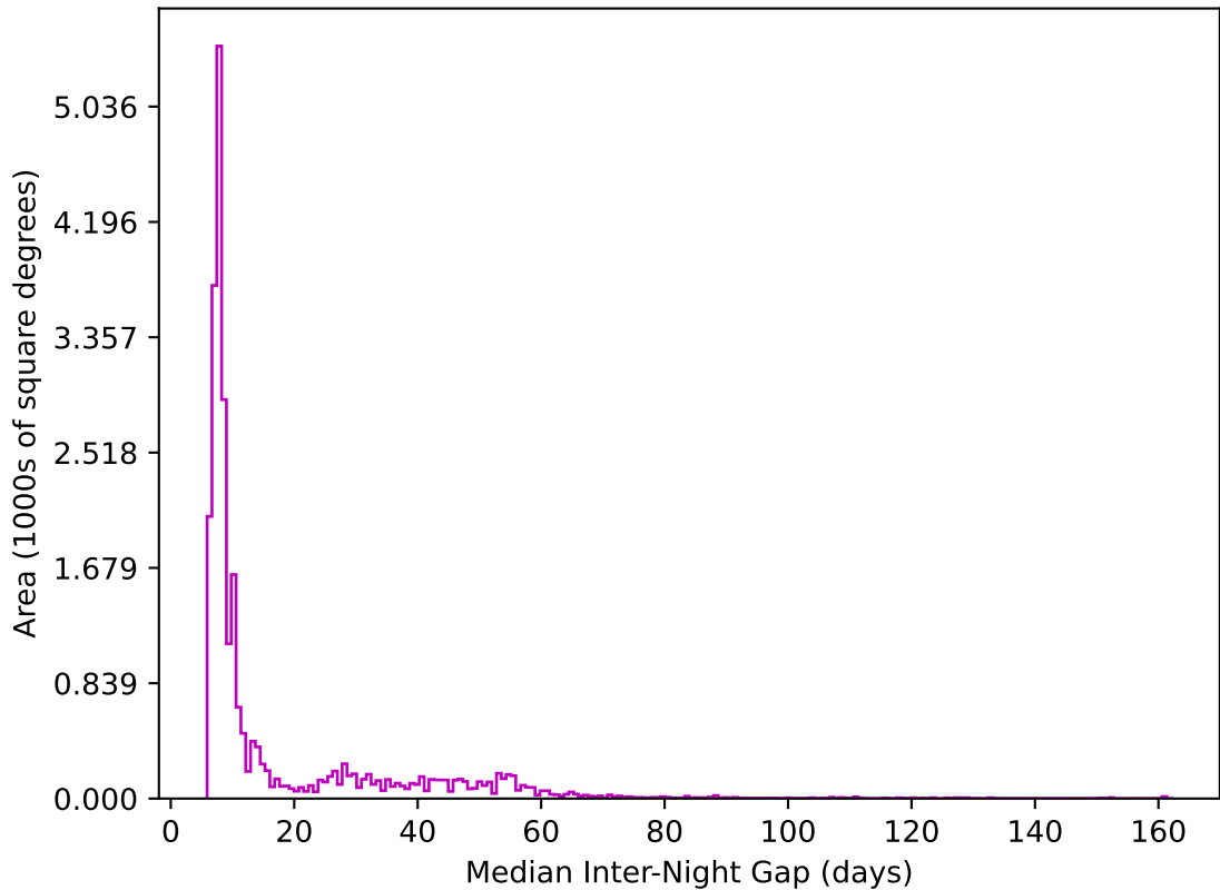
extra_ss_neo2_v3.4_10yrs All sky z band: Median Inter-Night Gap
