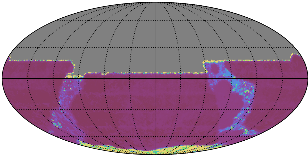
extra_ss_neo2_v3.4_10yrs All sky y band: Median Inter-Night Gap
