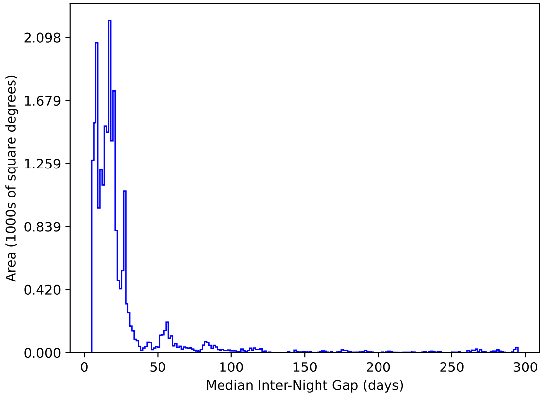
extra_ss_neo2_v3.4_10yrs All sky y band: Median Inter-Night Gap
