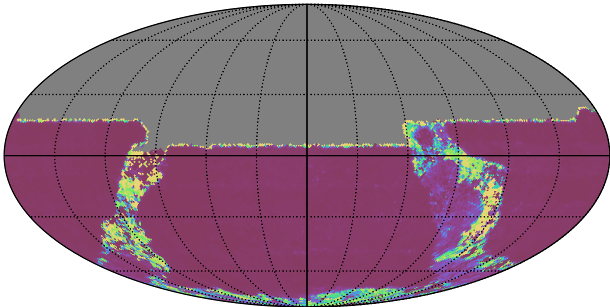
extra_ss_neo2_v3.4_10yrs All sky u band: Median Inter-Night Gap
