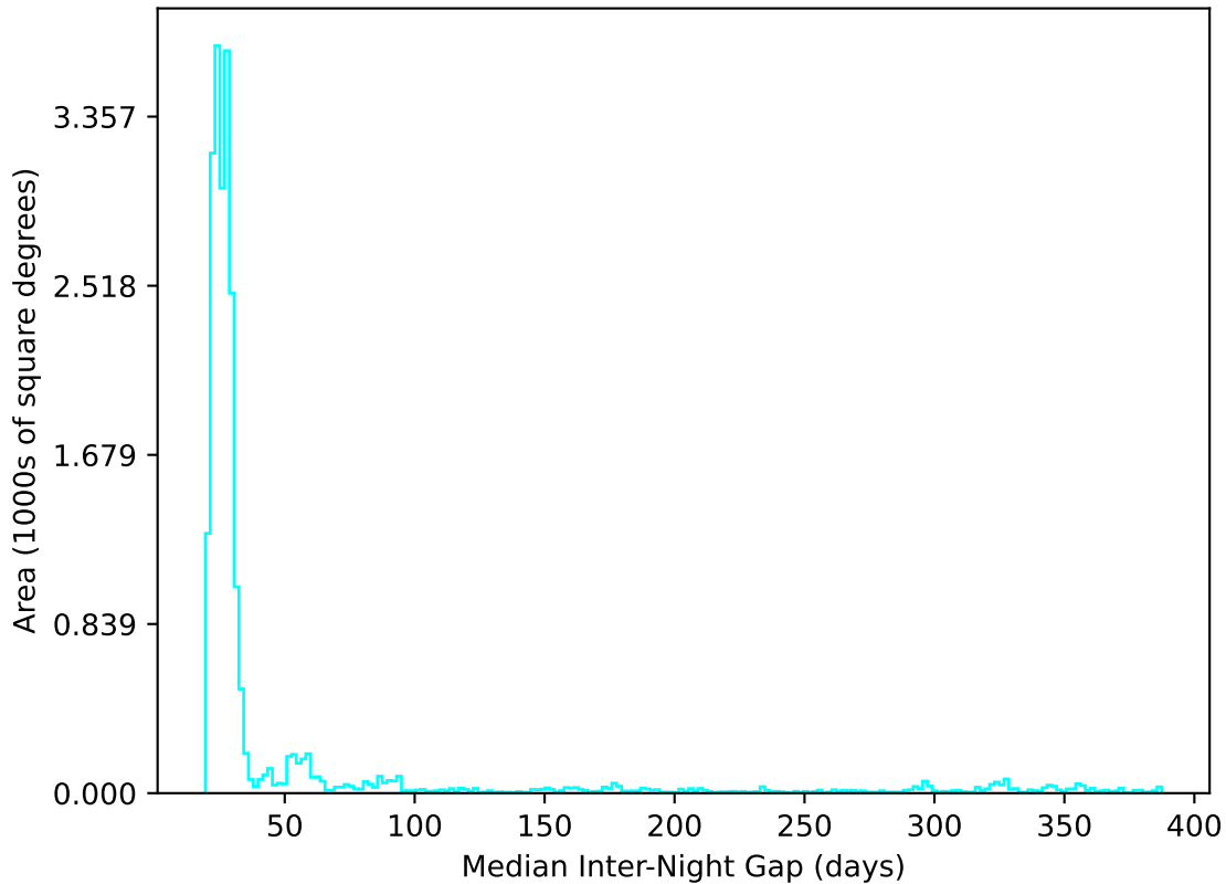
extra_ss_neo2_v3.4_10yrs All sky u band: Median Inter-Night Gap
