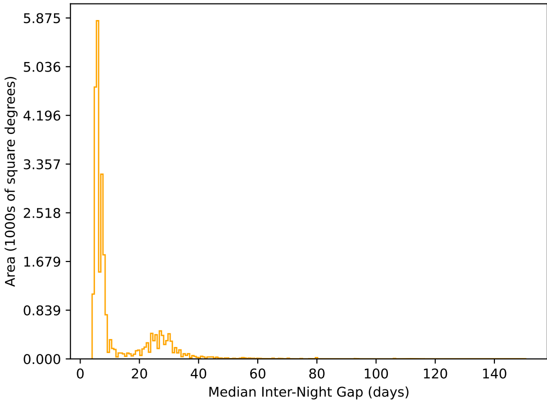
extra_ss_neo2_v3.4_10yrs All sky r band: Median Inter-Night Gap
