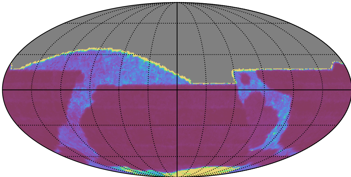
extra_ss_neo2_v3.4_10yrs All sky i band: Median Inter-Night Gap
