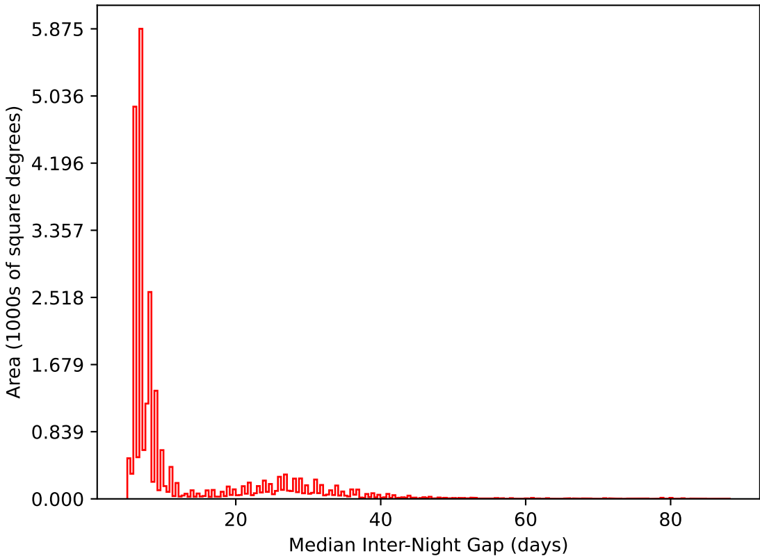
extra_ss_neo2_v3.4_10yrs All sky i band: Median Inter-Night Gap
