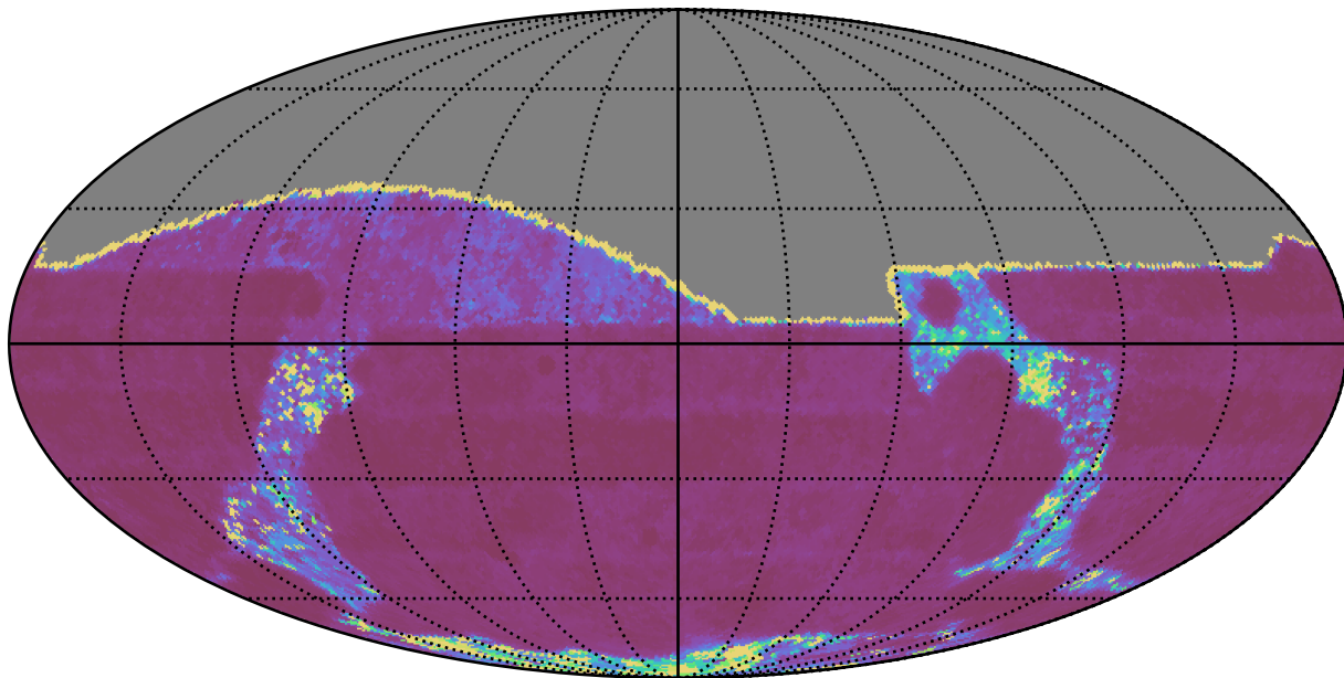
extra_ss_neo2_v3.4_10yrs All sky g band: Median Inter-Night Gap
