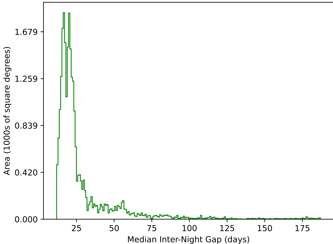
extra_ss_neo2_v3.4_10yrs All sky g band: Median Inter-Night Gap
