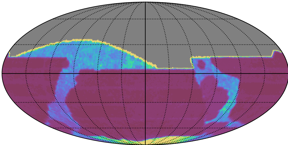
extra_ss_neo2_v3.4_10yrs All sky all bands: Median Inter-Night Gap
