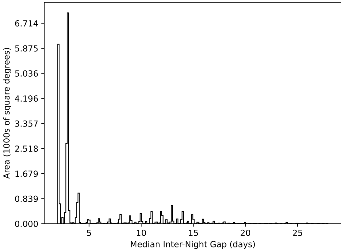
extra_ss_neo2_v3.4_10yrs All sky all bands: Median Inter-Night Gap
