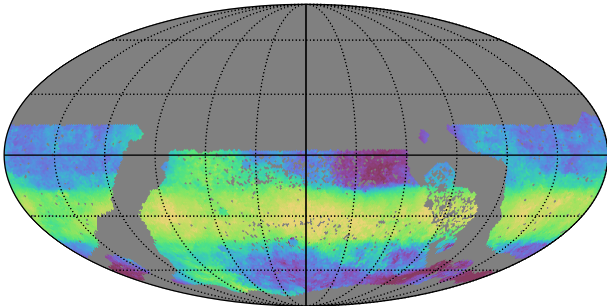
extra_ss_neo2_v3.4_10yrs WFD z band: Median HA
