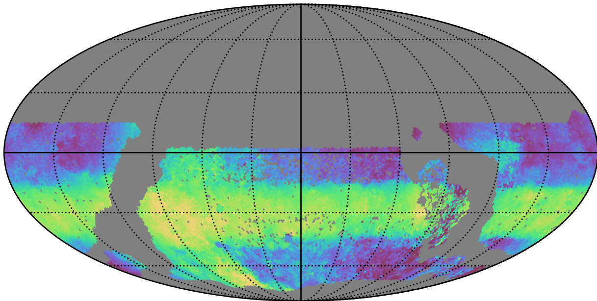
extra_ss_neo2_v3.4_10yrs WFD u band: Median HA
