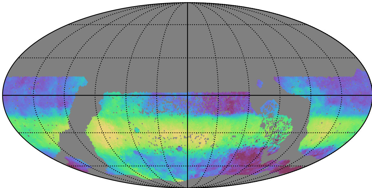
extra_ss_neo2_v3.4_10yrs WFD r band: Median HA
