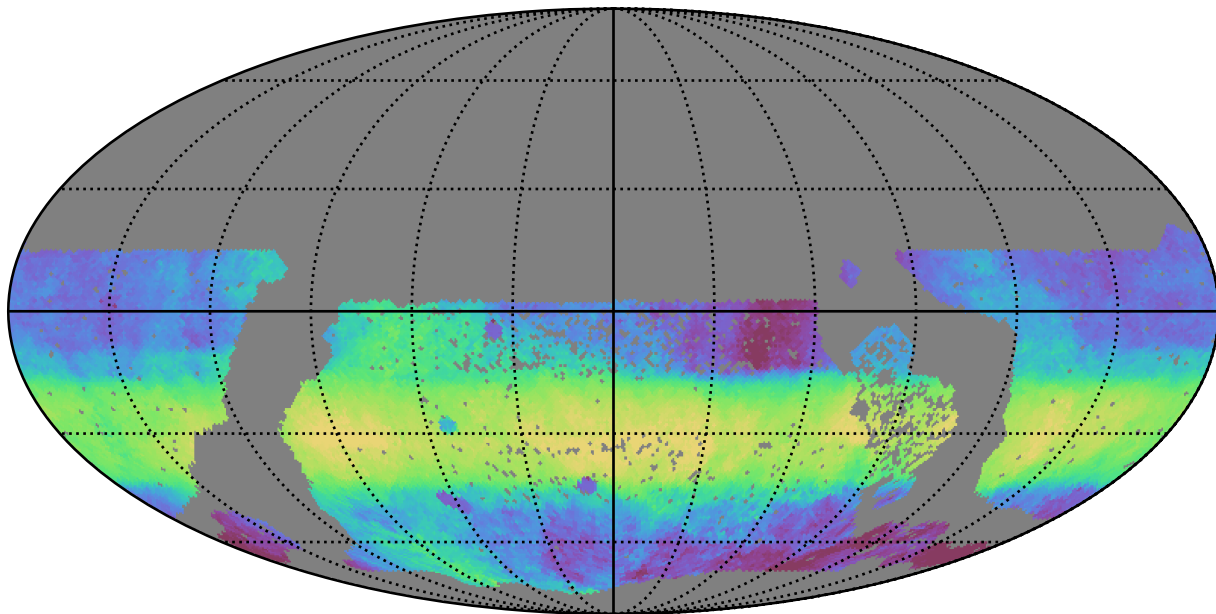
extra_ss_neo2_v3.4_10yrs WFD i band: Median HA
