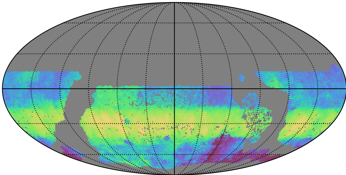
extra_ss_neo2_v3.4_10yrs WFD g band: Median HA
