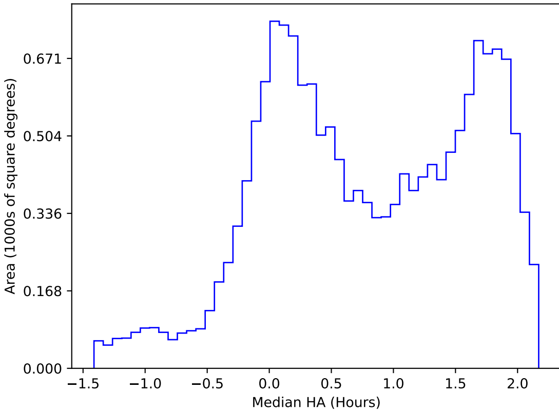
extra_ss_neo2_v3.4_10yrs WFD g band: Median HA
