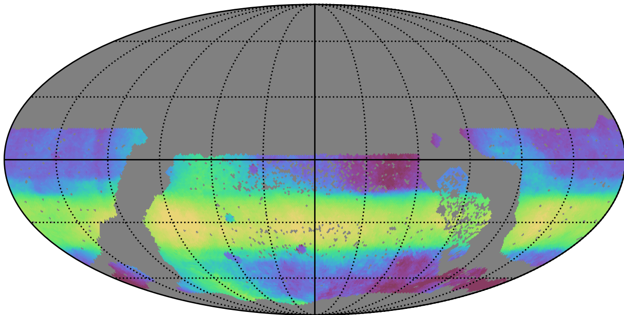
extra_ss_neo2_v3.4_10yrs WFD all bands: Median HA
