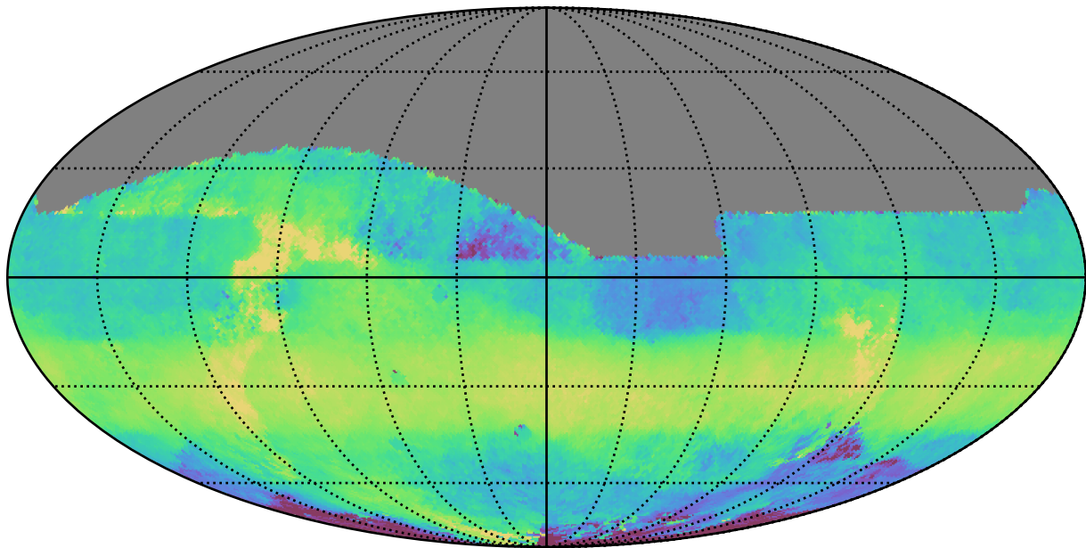
extra_ss_neo2_v3.4_10yrs All sky z band: Median HA
