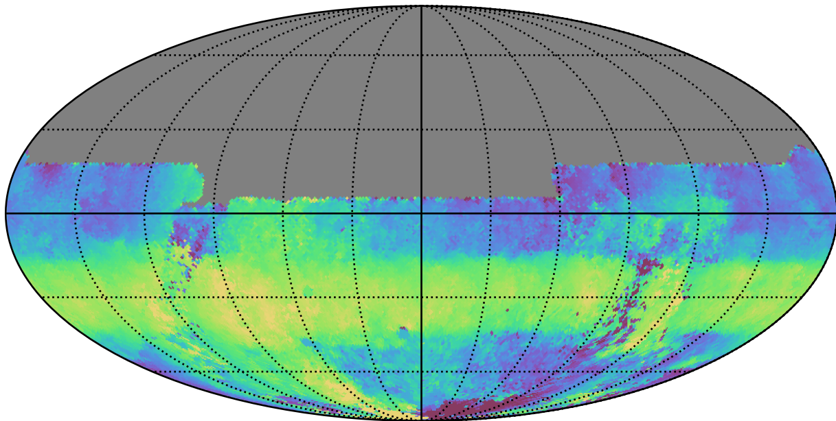
extra_ss_neo2_v3.4_10yrs All sky u band: Median HA
