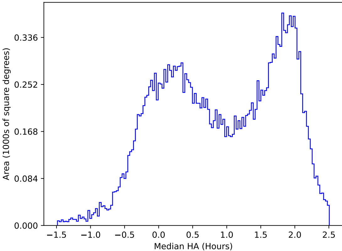
extra_ss_neo2_v3.4_10yrs All sky u band: Median HA
