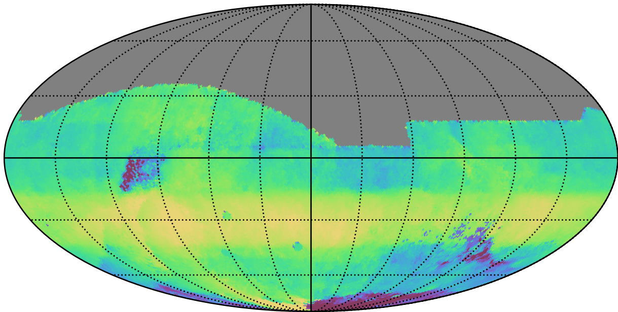
extra_ss_neo2_v3.4_10yrs All sky r band: Median HA
