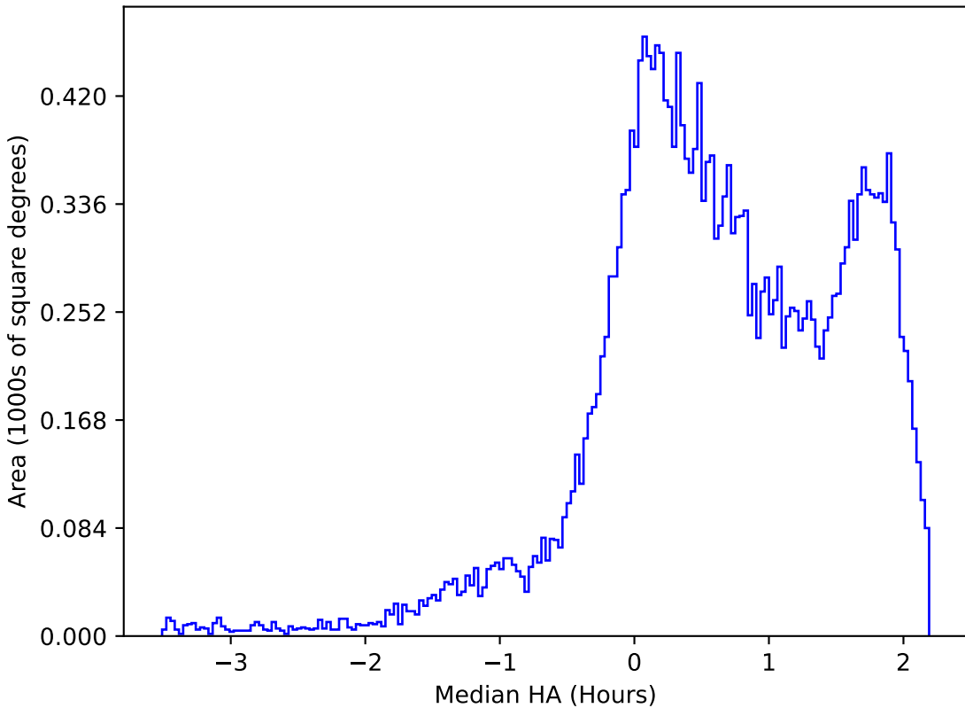
extra_ss_neo2_v3.4_10yrs All sky g band: Median HA
