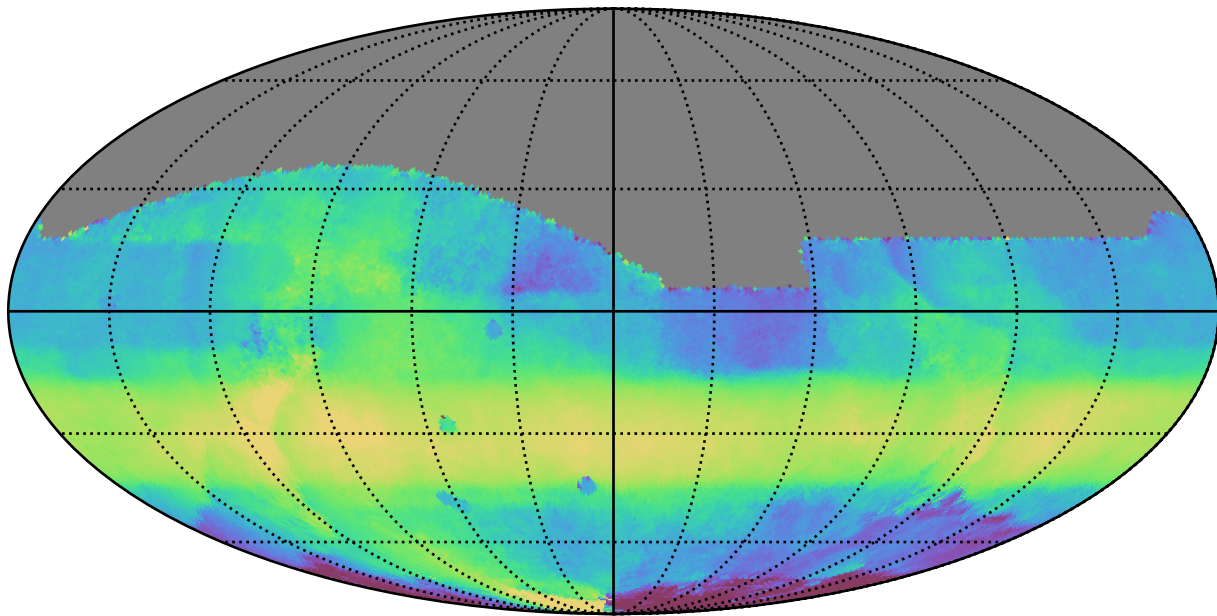
extra_ss_neo2_v3.4_10yrs All sky all bands: Median HA
