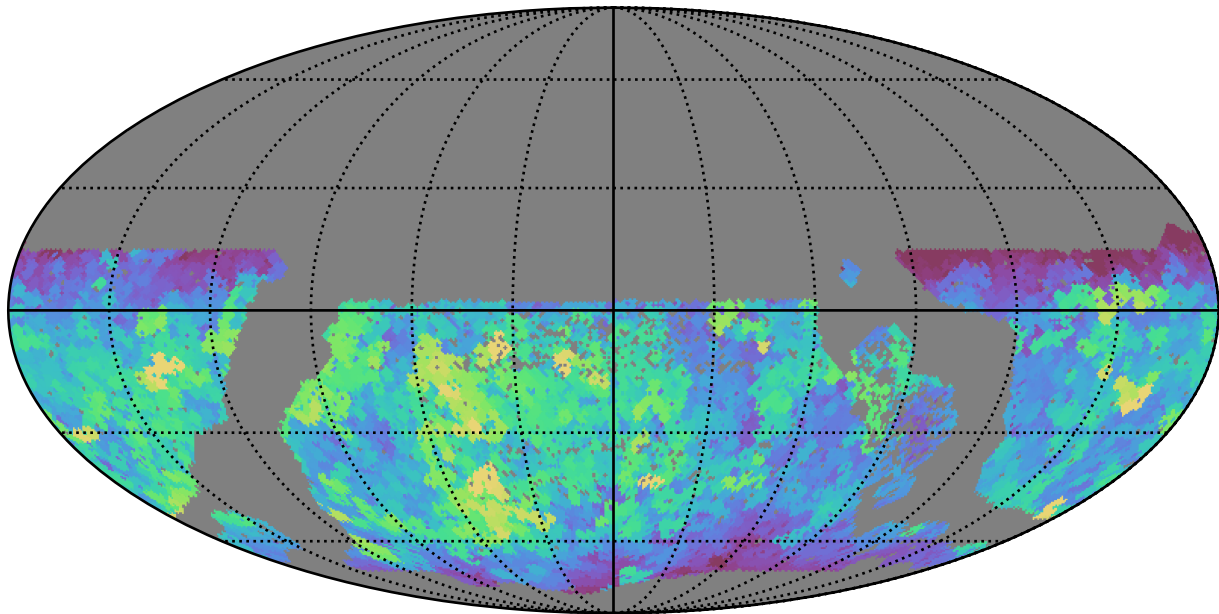
extra_ss_neo2_v3.4_10yrs WFD r band: Max saturation_mag
