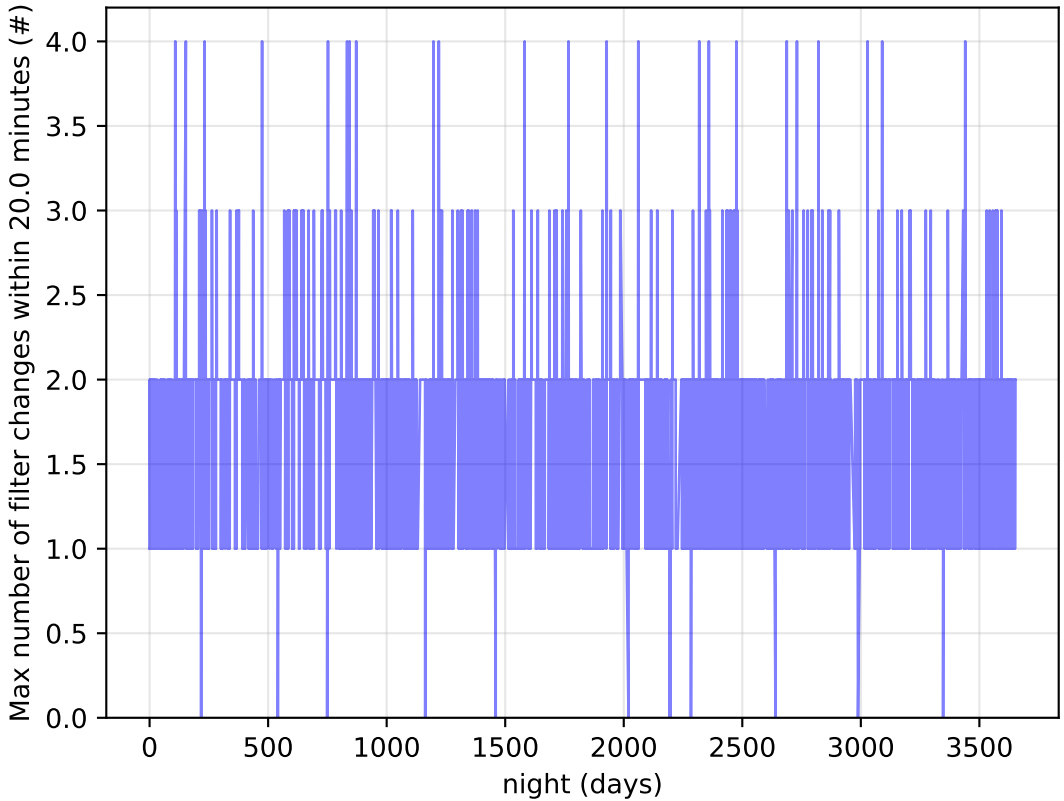
extra_ss_neo2_v3.4_10yrs Per Night: Max number of filter changes within 20.0 minutes
