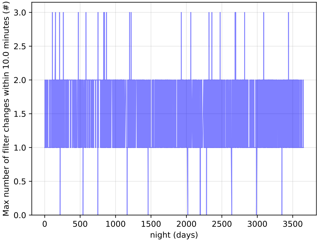
extra_ss_neo2_v3.4_10yrs Per Night: Max number of filter changes within 10.0 minutes
