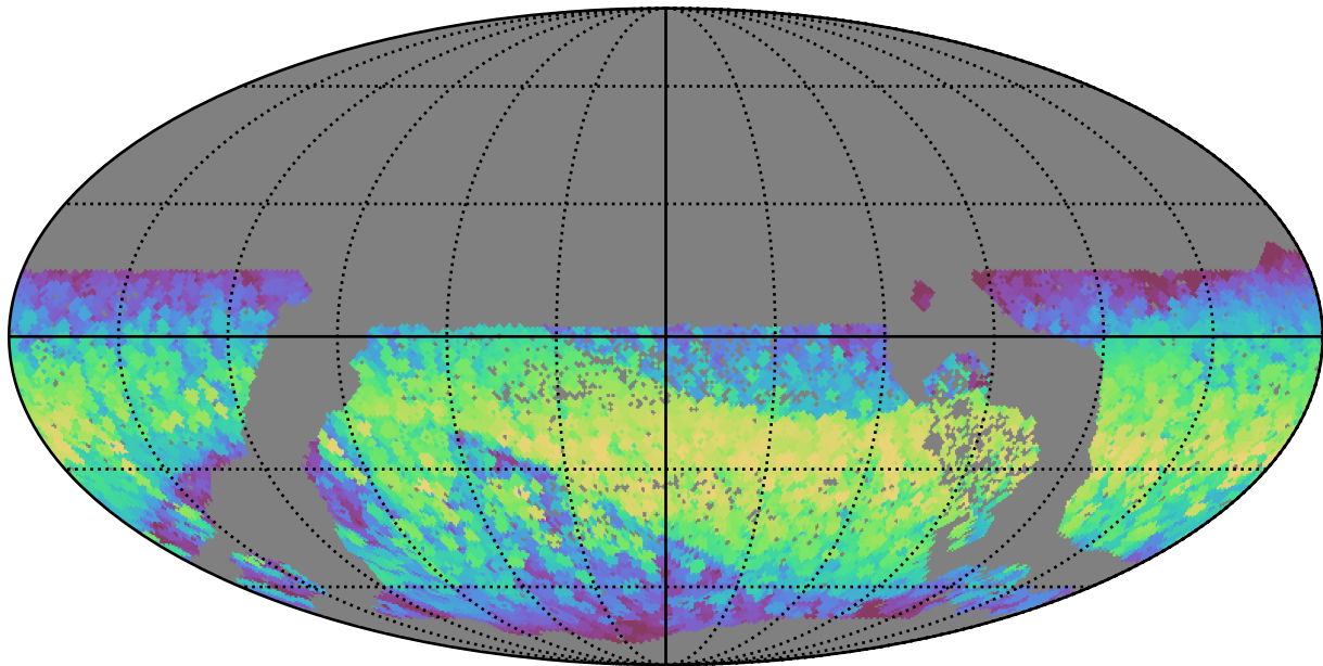
extra_ss_neo2_v3.4_10yrs WFD all bands: Max normairmass
