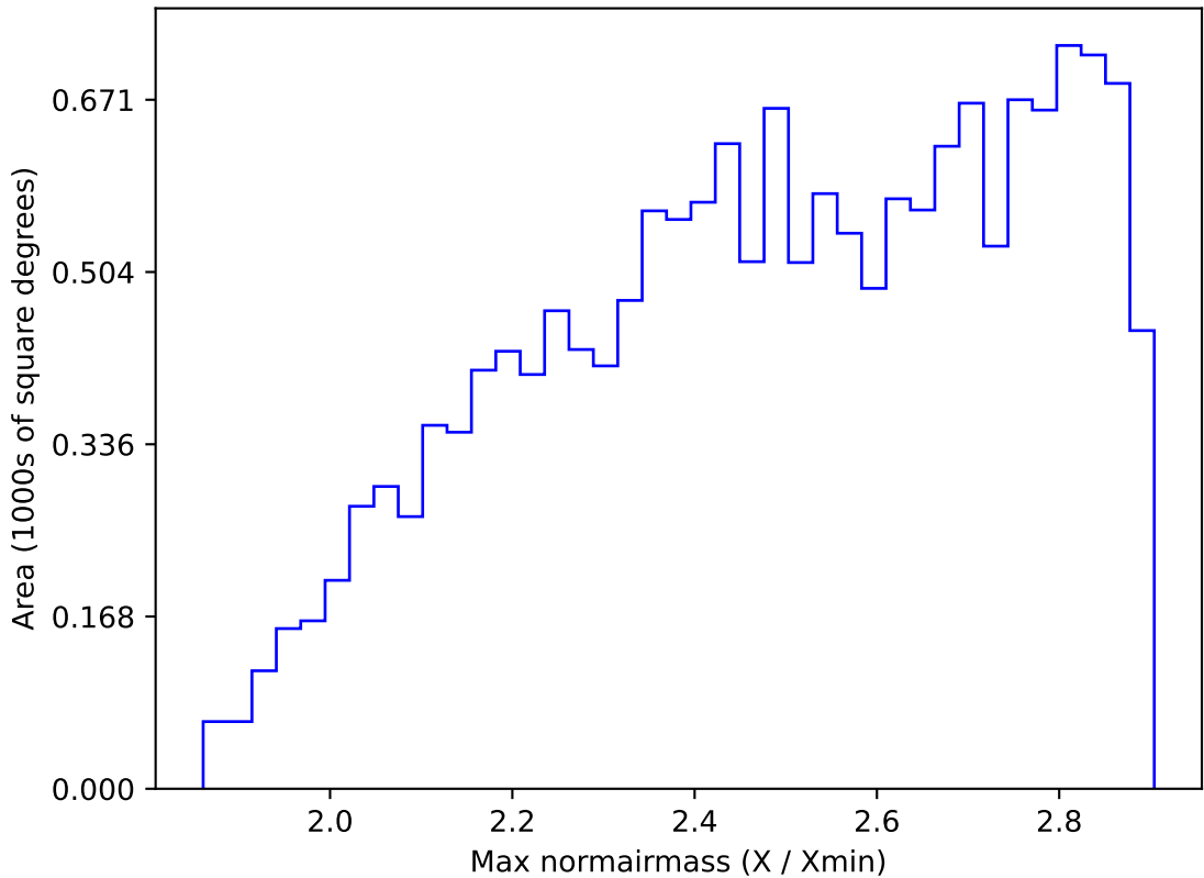
extra_ss_neo2_v3.4_10yrs WFD all bands: Max normairmass
