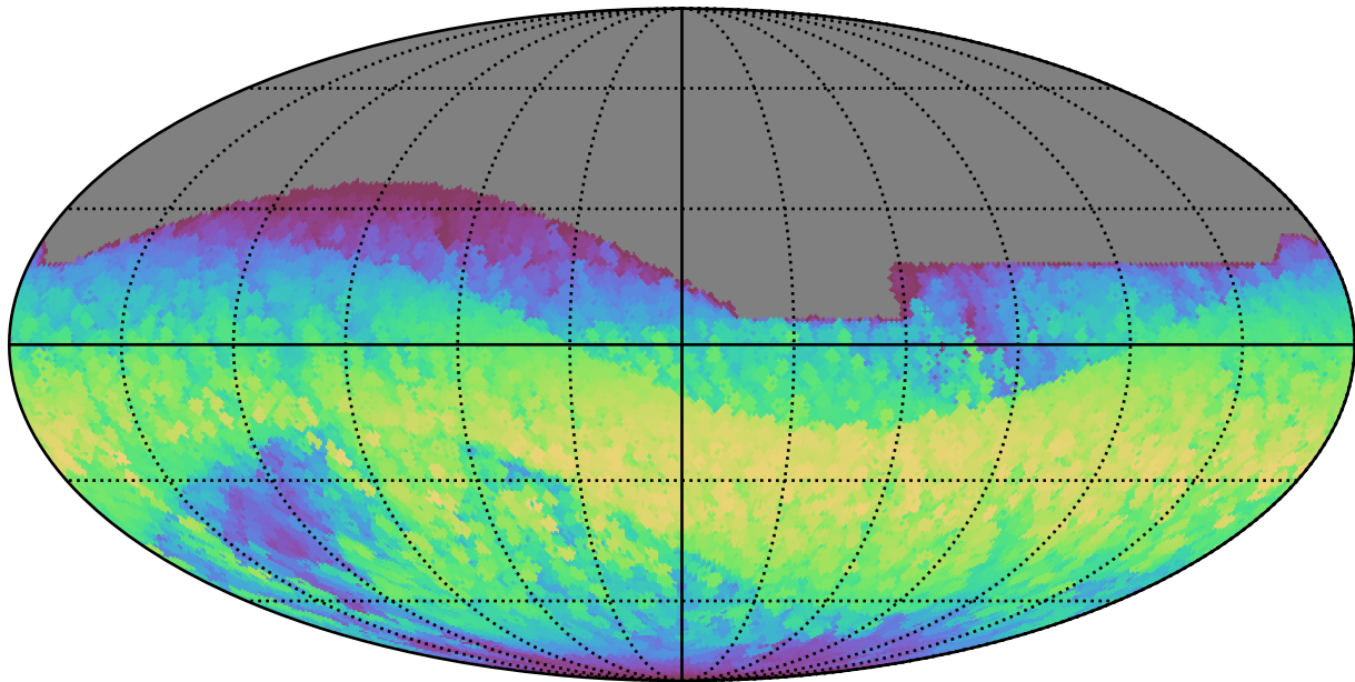
extra_ss_neo2_v3.4_10yrs All sky all bands: Max normairmass
