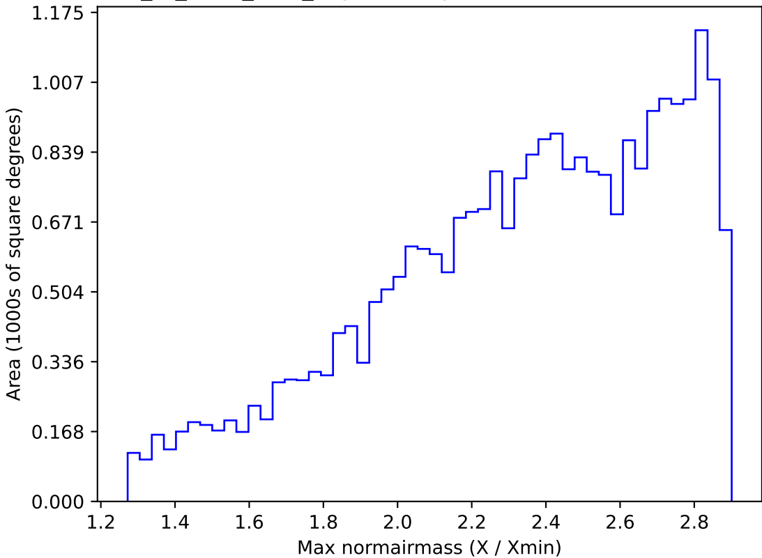
extra_ss_neo2_v3.4_10yrs All sky all bands: Max normairmass
