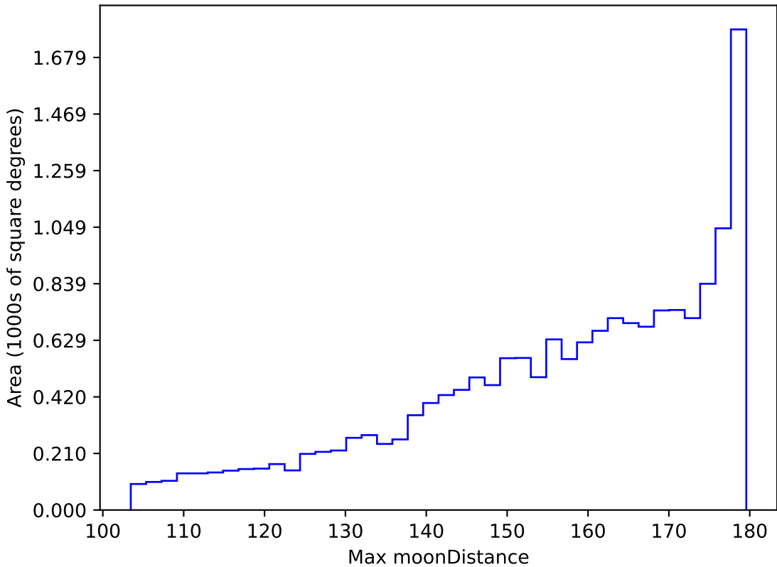
extra_ss_neo2_v3.4_10yrs WFD all bands: Max moonDistance
