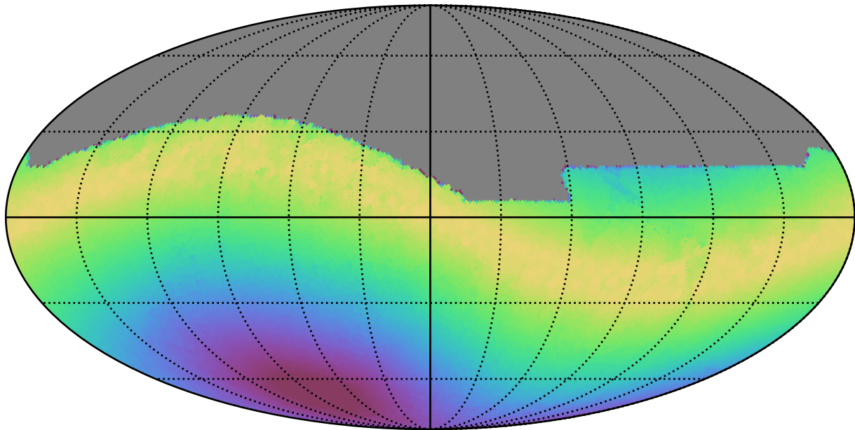
extra_ss_neo2_v3.4_10yrs All sky all bands: Max moonDistance
