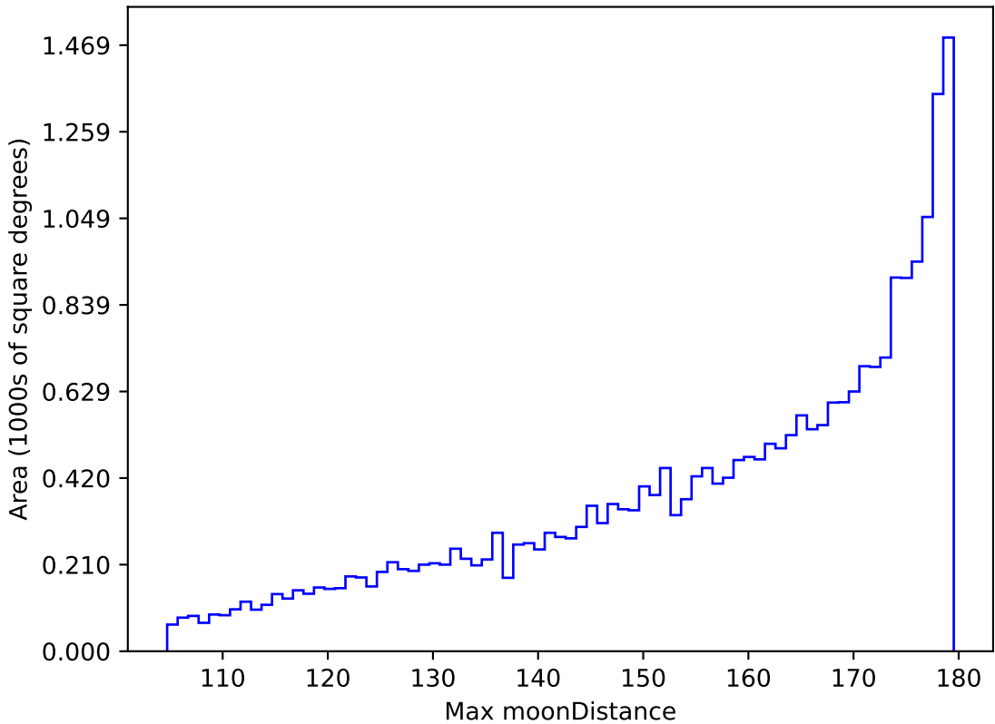
extra_ss_neo2_v3.4_10yrs All sky all bands: Max moonDistance
