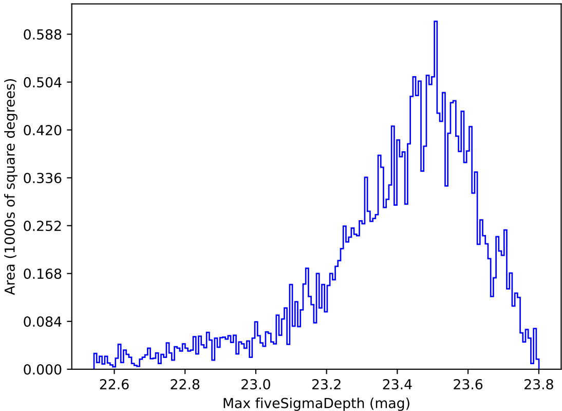
extra_ss_neo2_v3.4_10yrs Yr 1 z band: Max fiveSigmaDepth
