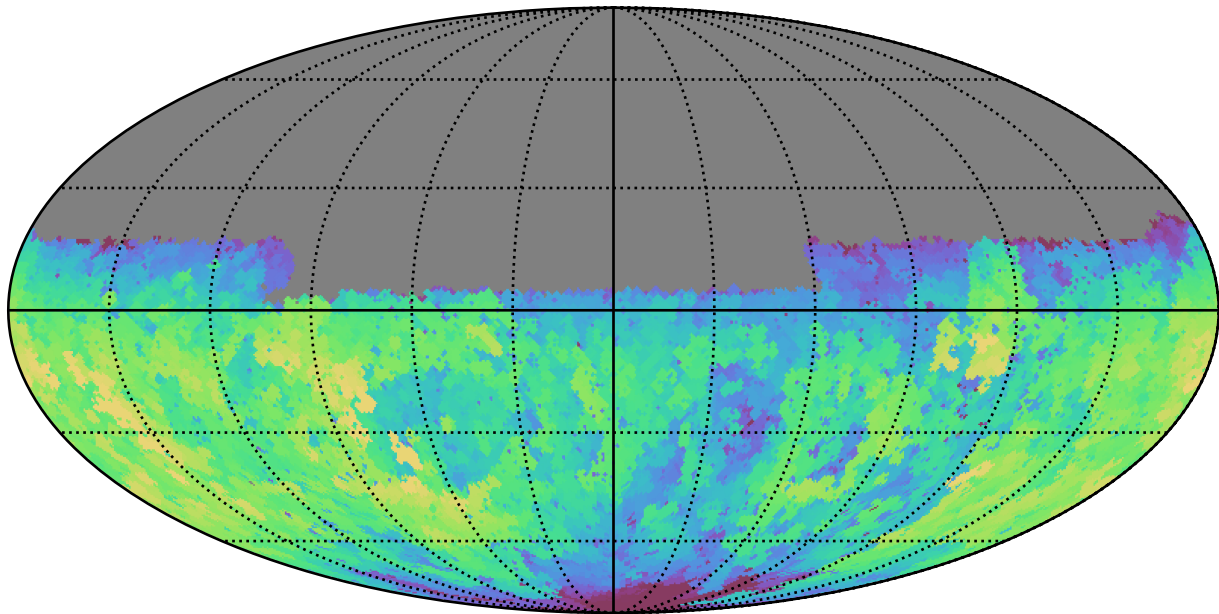
extra_ss_neo2_v3.4_10yrs Yr 1 u band: Max fiveSigmaDepth
